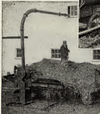
John Deere Roughage Mill and Feed Grinder
