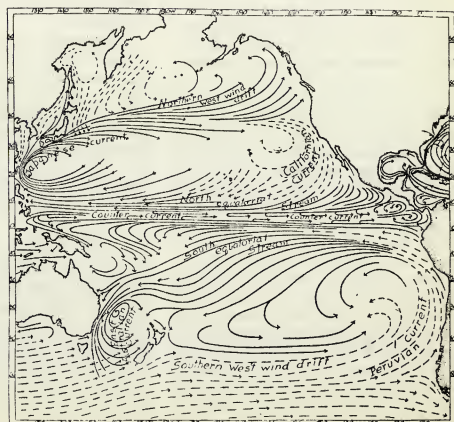
FIG. 39. GENERAL SCHEME OF THE CIRCULATION IN THE PACIFIC OCEAN.
